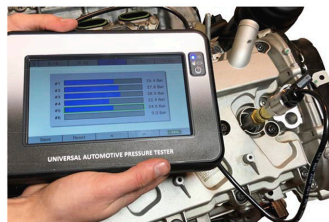
Gasoline compression
